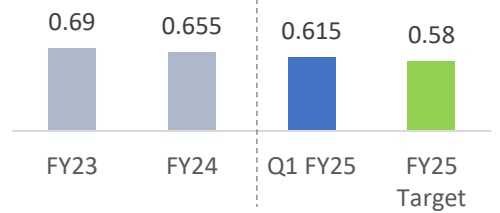
NOx Emissions (kg/MWh)
